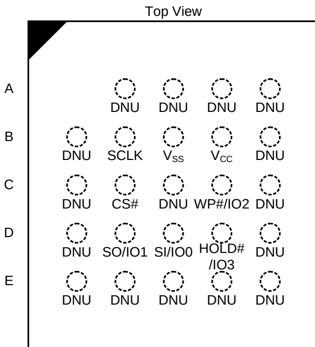
Figure 2: Pin Map
