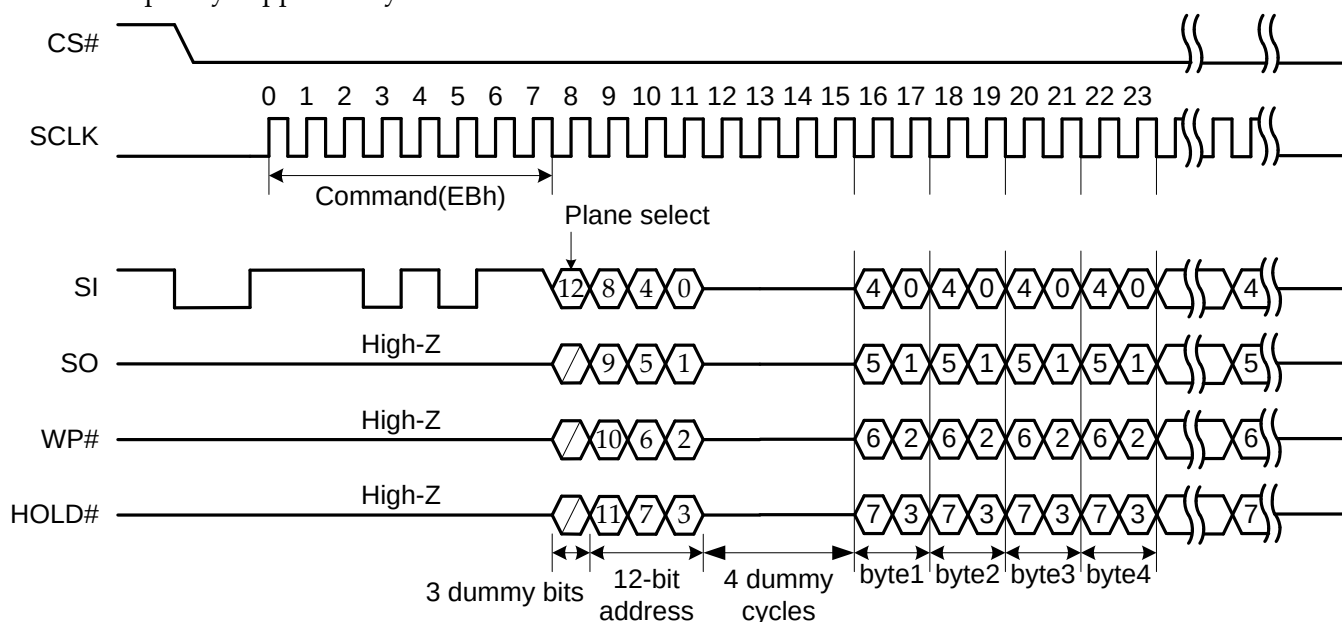
Figure 14: Read From Cache Quad IO (EBh) Command Timing
