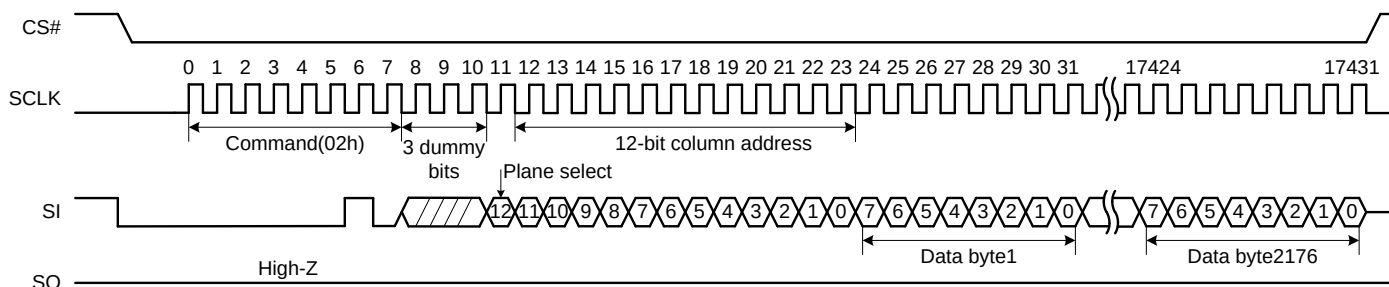
Figure 17: Program Load (02h) Command Timing
