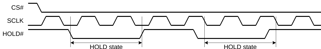
Figure 3: HOLD Condition
