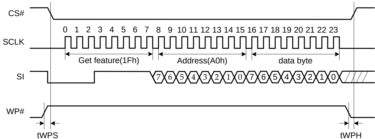
Figure 31: WP# Timing
