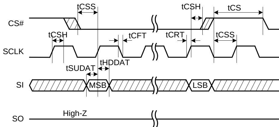
Figure 32: Serial Input Timing
