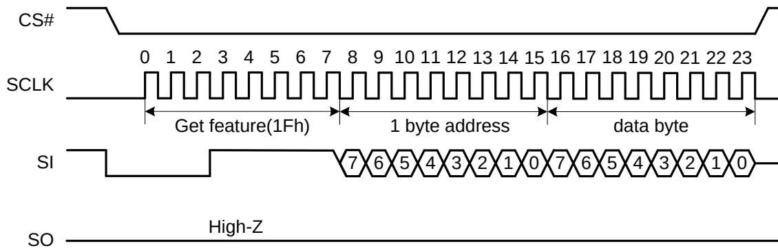
Figure 23: Set Features (1Fh) Command Timing
