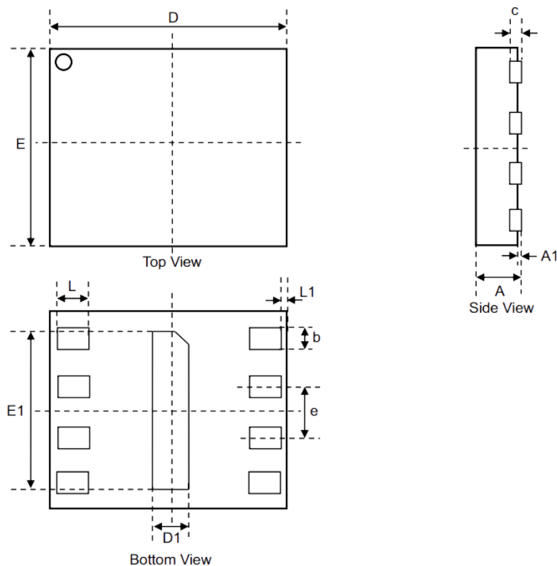
Figure 49: USON8(2*3mm) Package
