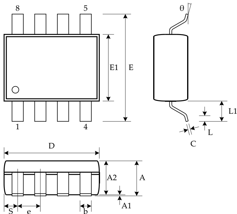
Figure 40: SOP8(150mil) Package
