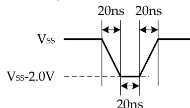
Figure 34: Maximum Positive / Negative Overshoot Timing Diagram
