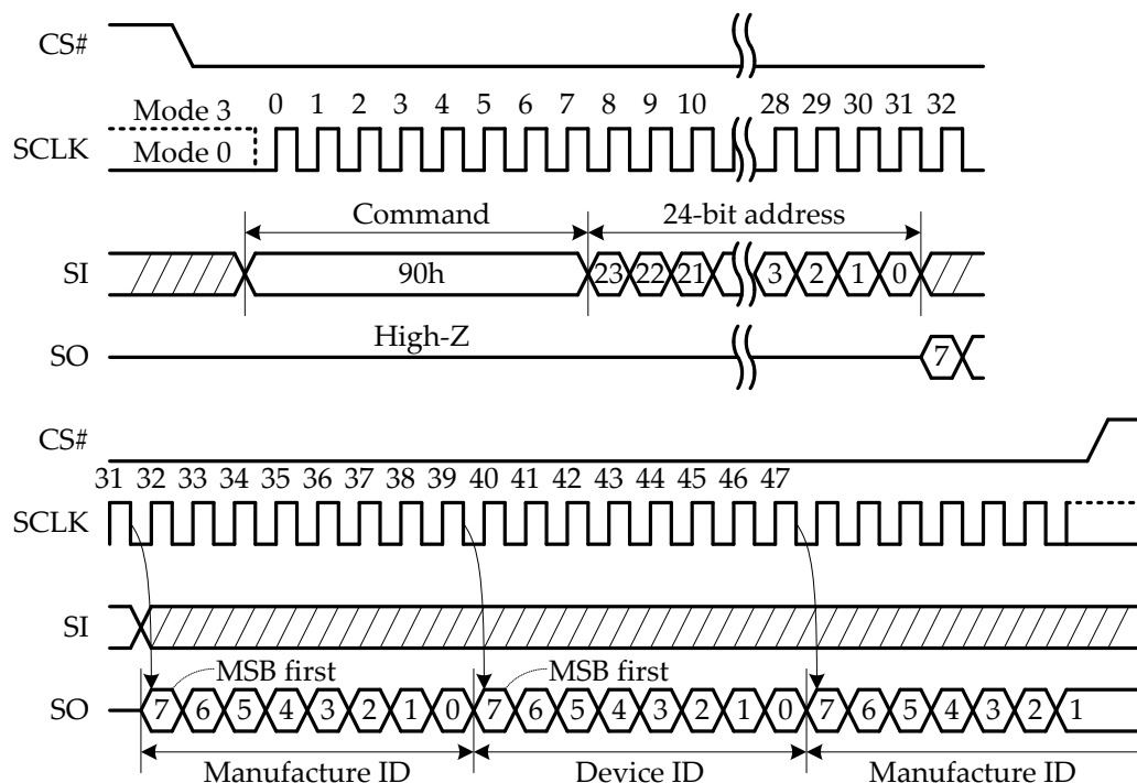
Figure 24: Read Manufacturer ID / Device ID (REMS) (90h) Command Sequence
