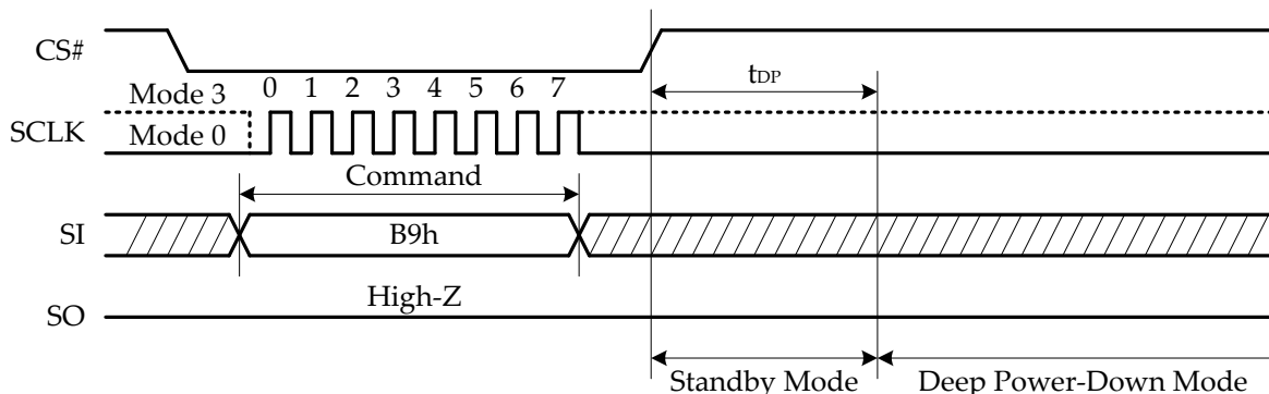
Figure 20: Deep Power-Down (DP) (B9h) Command Sequence
