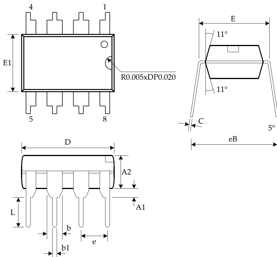
Figure 42: DIP8(300mil) Package
