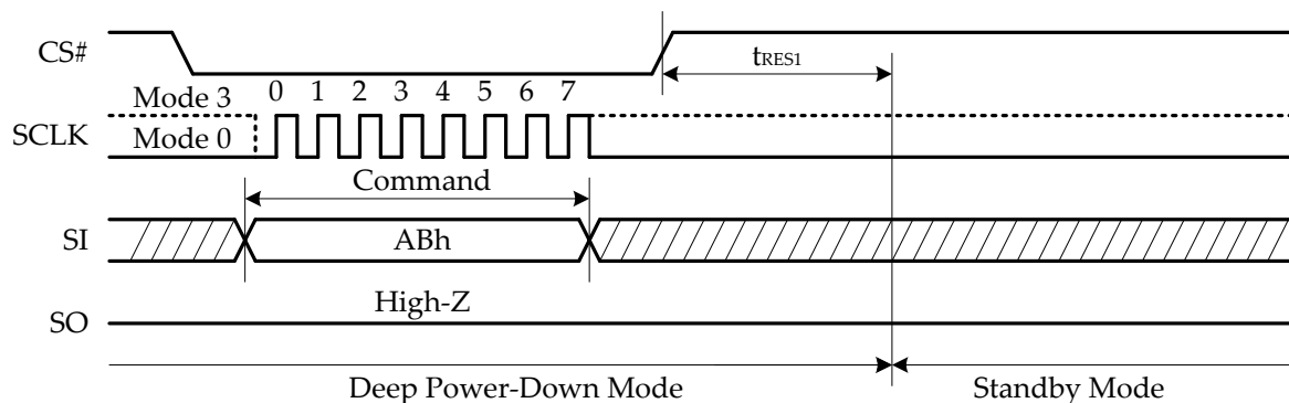
Figure 22: Release Power-Down (ABh) Command Sequence
