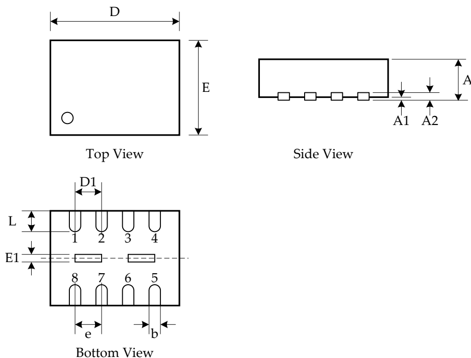
Figure 48: USON8(4*3mm) Package
