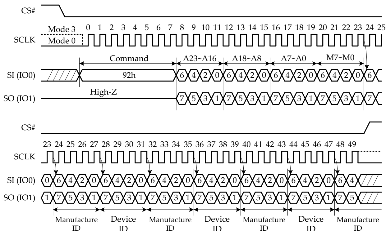
Figure 25: Dual I/O Read Manufacture ID / Device ID (92h) Command Sequence
