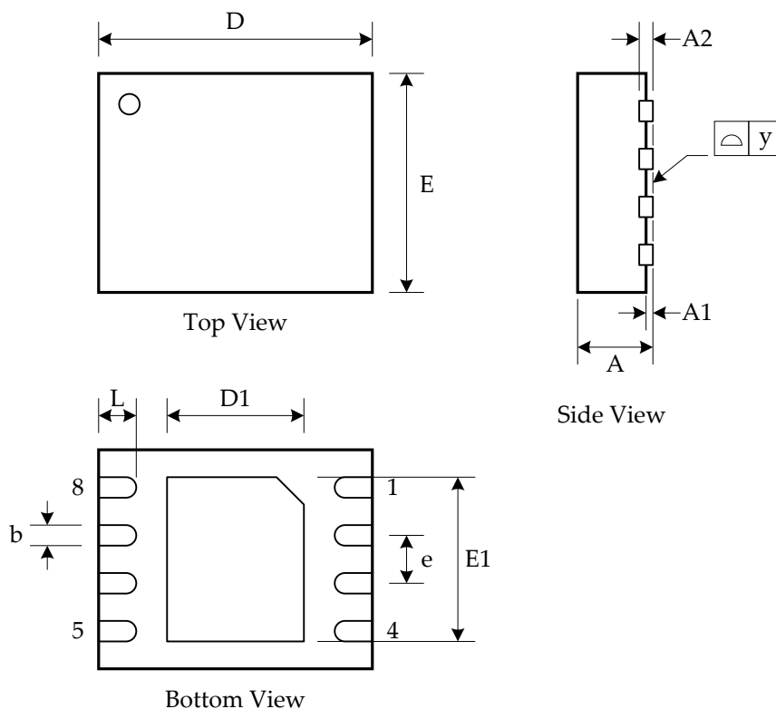
Figure 43: WSON8(6*5mm) Package
