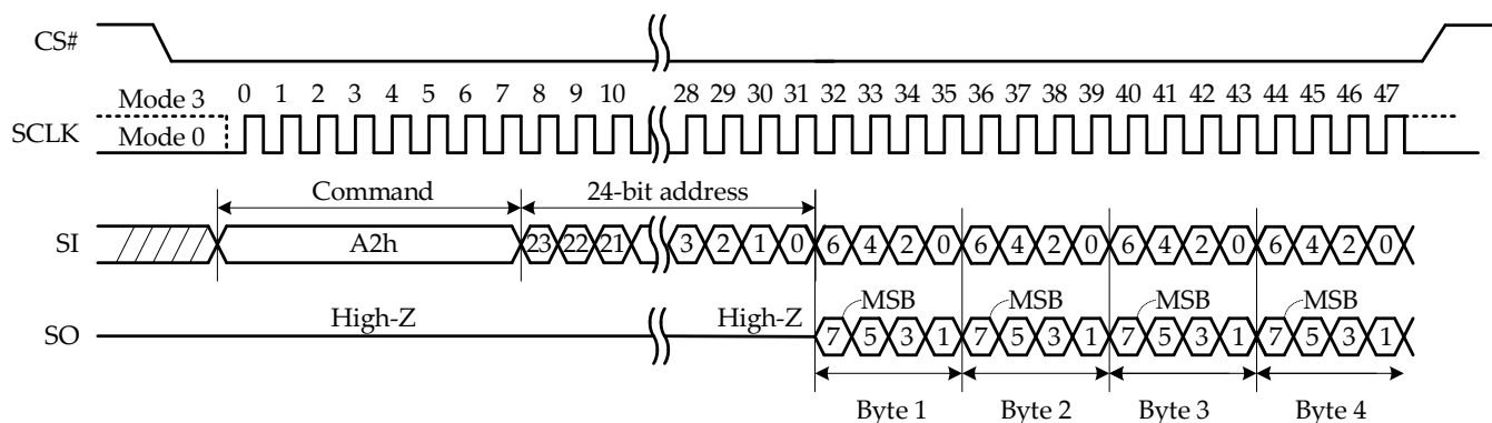
Figure 14: Dual Input Page Program (A2h) Command Sequence
