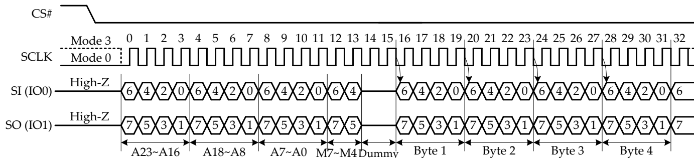
Figure 12: Dual I/O Fast Read (BBh) Command Sequence
