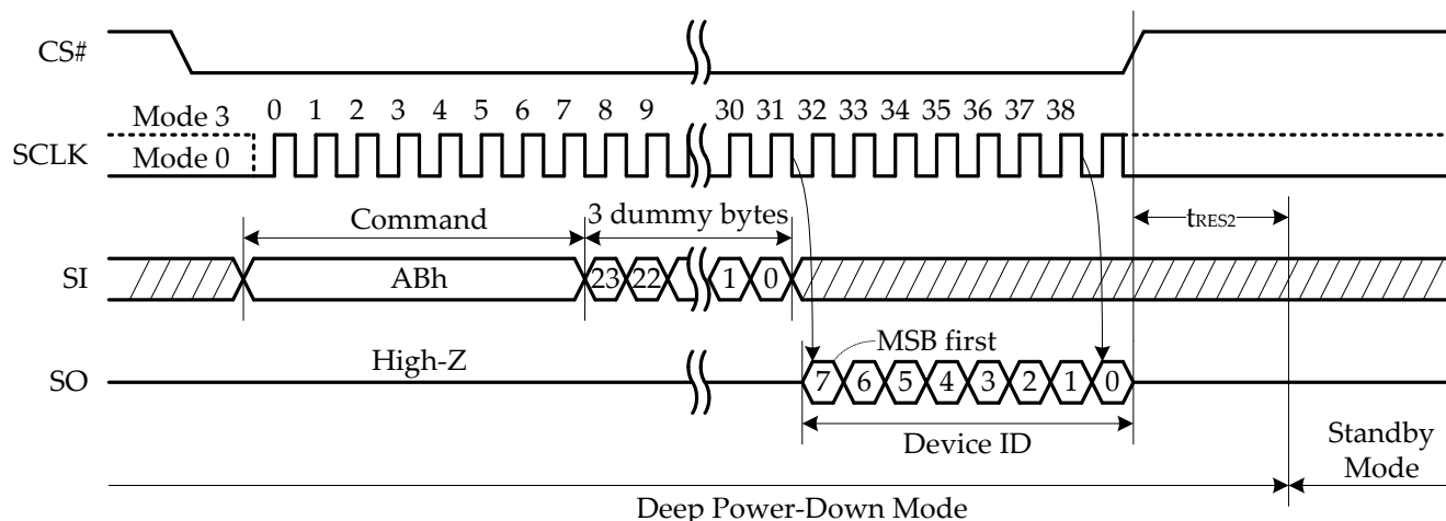
Figure 23: Release Power-Down and Read Device ID (ABh) Command Sequence
