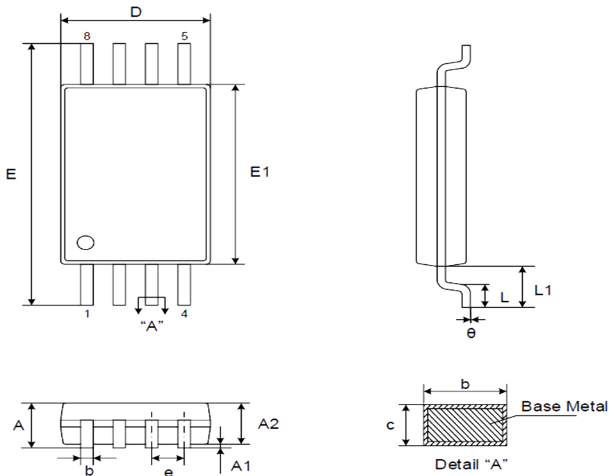
Figure 41: SOP8(150mil) Package
