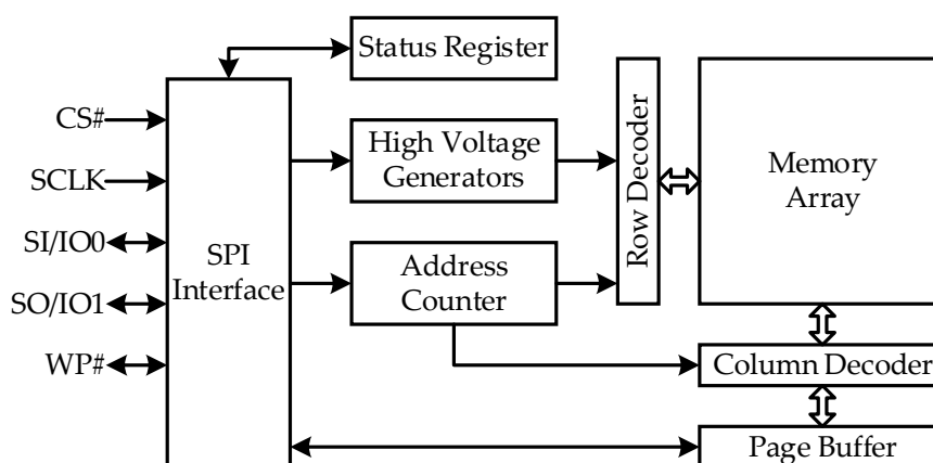
Figure 1: NM25WD40A SPI Flash Block Diagram
