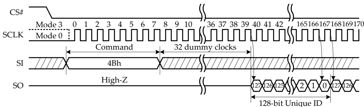
Figure 21: Read Unique ID (4Bh) Command Sequence
