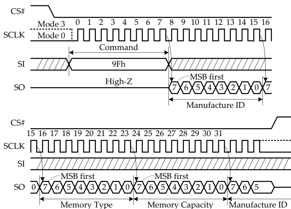
Figure 26: Read Identification (RDID) (9Fh) Command Sequence
