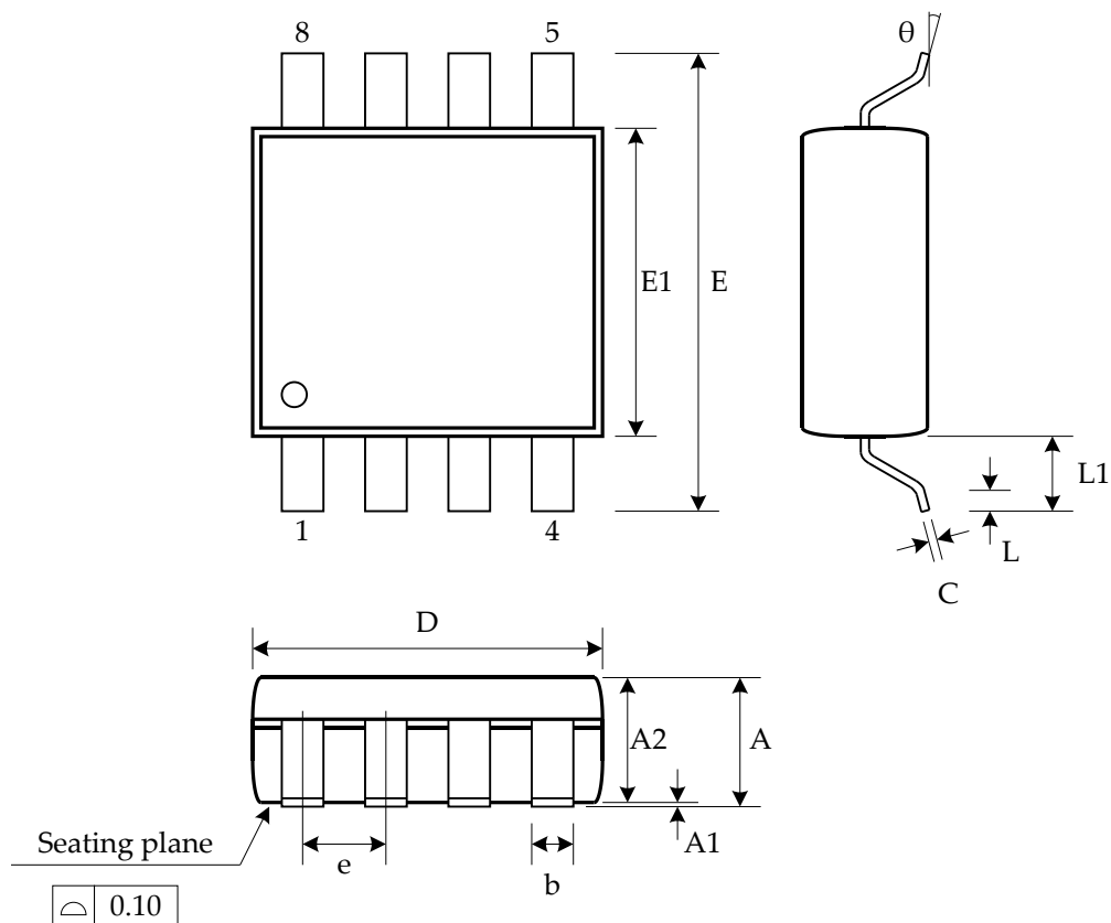
Figure 39: SOP8(208mil) Package
