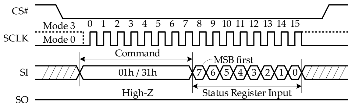
Figure 7: Write Status Register (WRSR) (01h or 31h) Command Sequence
