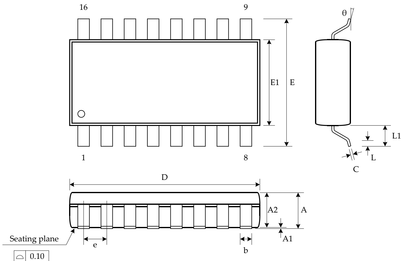
Figure 46: SOP16(300mil) Package
