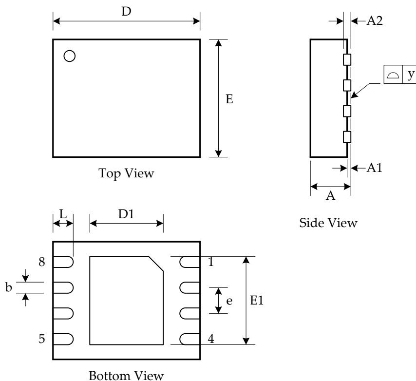
Figure 44: WSON8(8*6mm) Package
